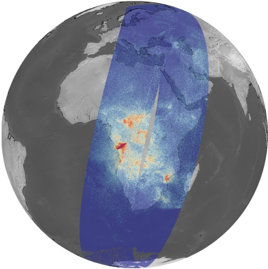
Formaldehyde 13 October 2025 0 350 700 \mu\text{mol}/\text{m}^2
