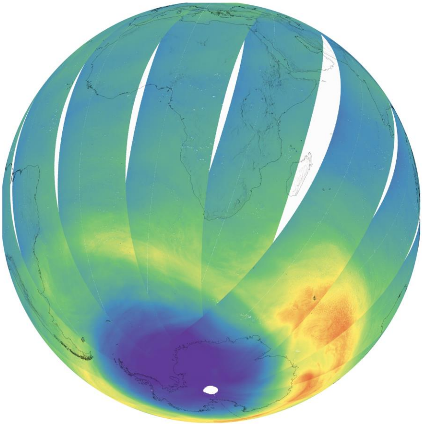
Ozone 13 October 2025 180 370 560 DU
